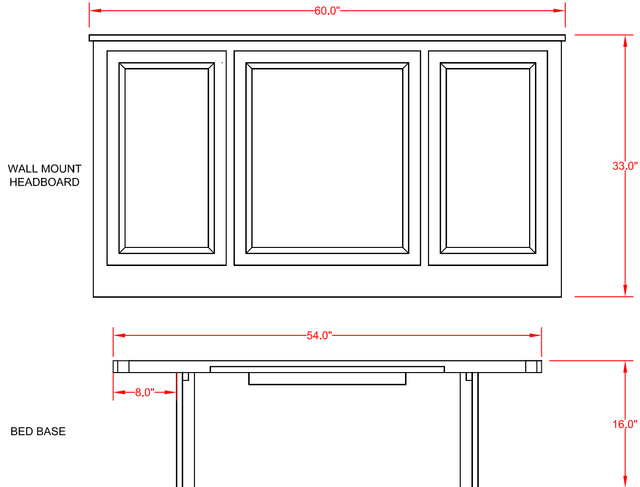
FRONT VIEW
