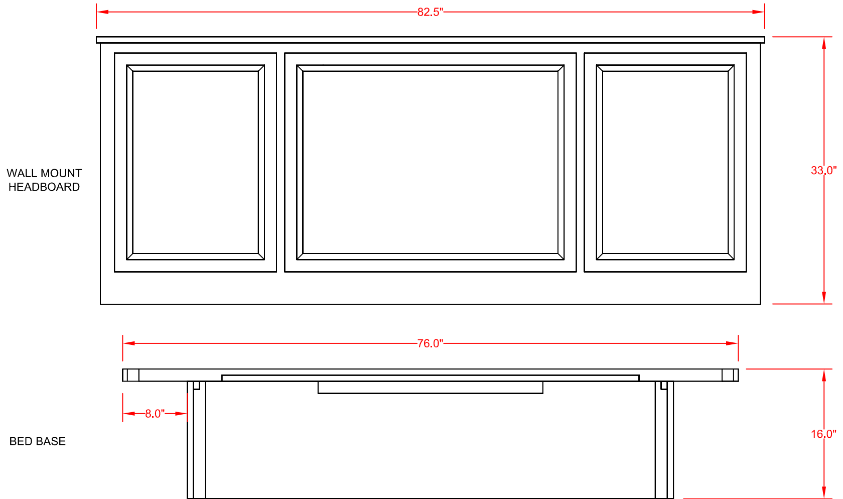
FRONT VIEW
